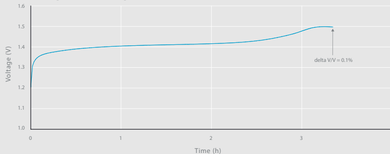
End of charge cut-off - charge at C/3
