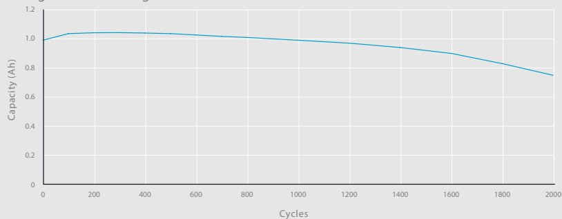
Charge at C/3 - discharge at 0.5 A
