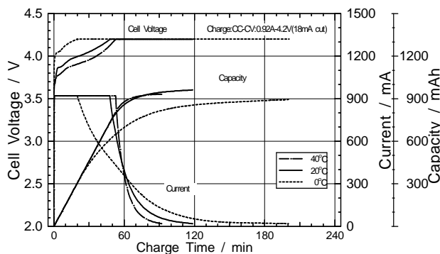
Charge characteristics
